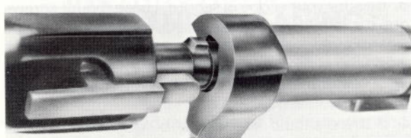
Photo #5: Square boss correctly positioned and about to be inserted in indexing groove.
