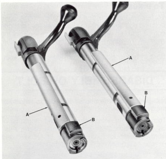
Photo #2: Photo shows (A) rotatable guide bar and (B) front locking lug. Bolt on right shows guide bar properly aligned with front locking lug. Bolt on left shows guide bar improperly aligned with front locking lug.
