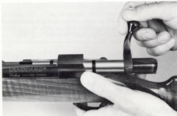
Photo #3: Depress release latch to remove bolt.
