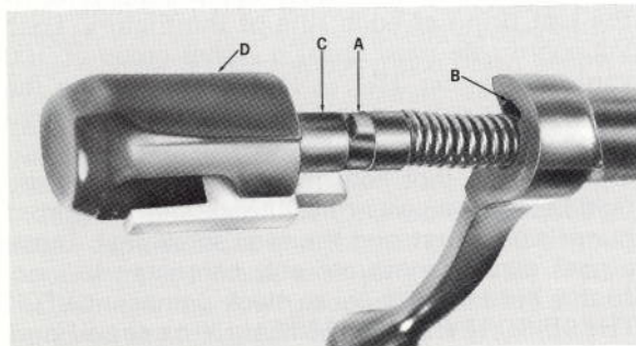
Photo #4: (A) Square boss, (B) Indexing groove, (C) Bolt sleeve shank, (D) Bolt sleeve.
