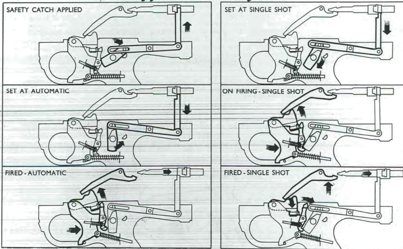
Trigger and Firing Action (Fig.16)
