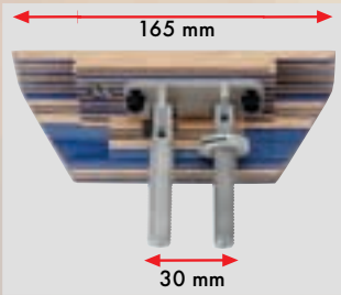
↑ Alu Backenausleger inkl. Backe, natur/blau. Alu cheek piece adjustment complete with cheek piece, natural/blue. Best.-Nr.: 700.3574
