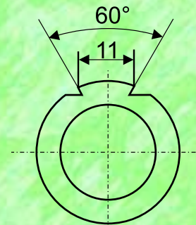
11 mm grooved receiver drilled and tapped for scope mounts.
