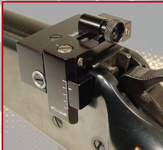
FP-94 SE SHOWN ON WINCHESTER 94 SIDE EJECT
