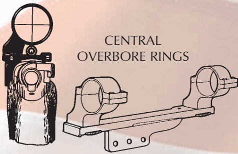
QC SIDE MOUNT - OFFSET - OR OVERBORE
