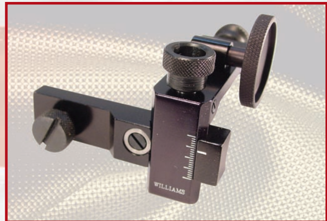
TARGET – FP (Low) Adjustable From .750" to 1.250" Above Centerline of Bore.
