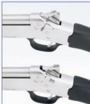
The manual safety prevents the hammer from striking the transfer bar mechanism.
