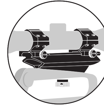
KWIK-SITE SEE-THRU MOUNT FOR M-16 & AR-15
