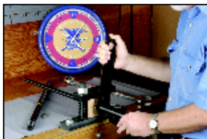
2. The barrel is clamped in the vise and the barrel nut is loosened.
