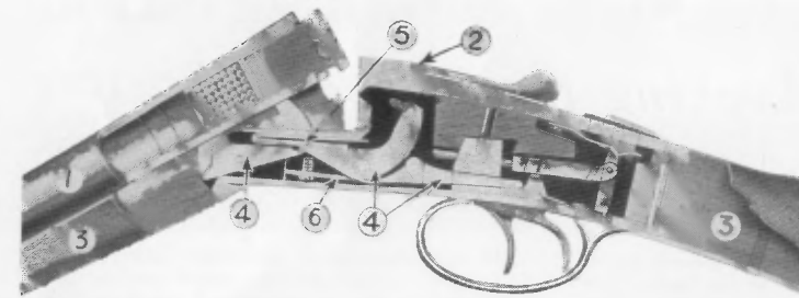
Section of the B.S.A. Shot Gun.
