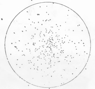
30 yards' range. Circle, 30ins. diameter. Left barrel, full choke.
