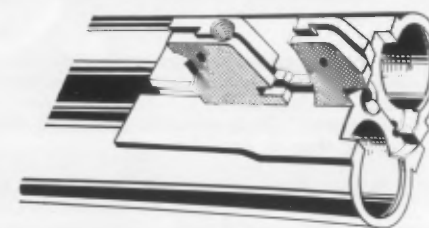
Showing method of dovetailing the barrels together with solid lumps.
