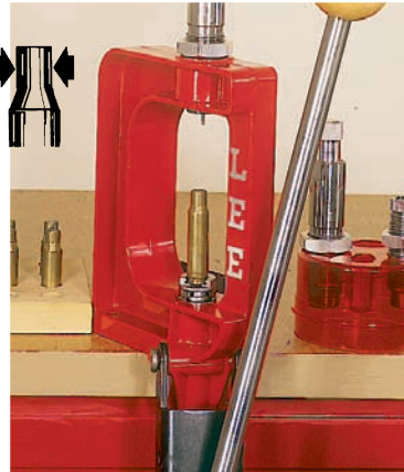
Remove spent primer and resize case
