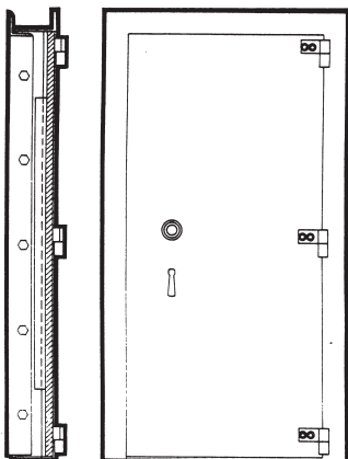
Vault Door: B Rate to TL-30 High Security Construction available
