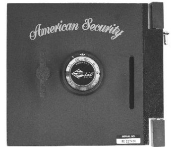
SUPER BRUTE "B" and "CB" Rate Slotted Square Hinged Door with 3/8" x 4" slot.
